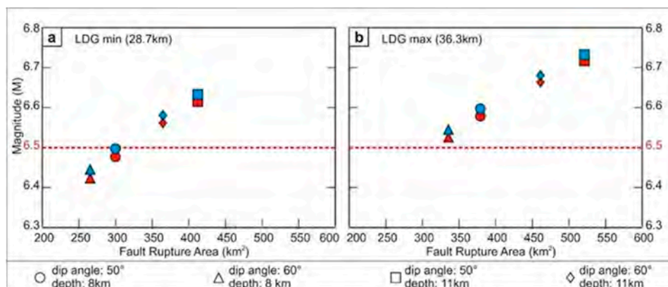
Figure 9. Earthquake magnitude estimates from Length of the Deforming Ground (LDG). (a) earthquake magnitude is estimated using LDG minimum, (b) earthquake magnitude is estimated using LDG maximum.
