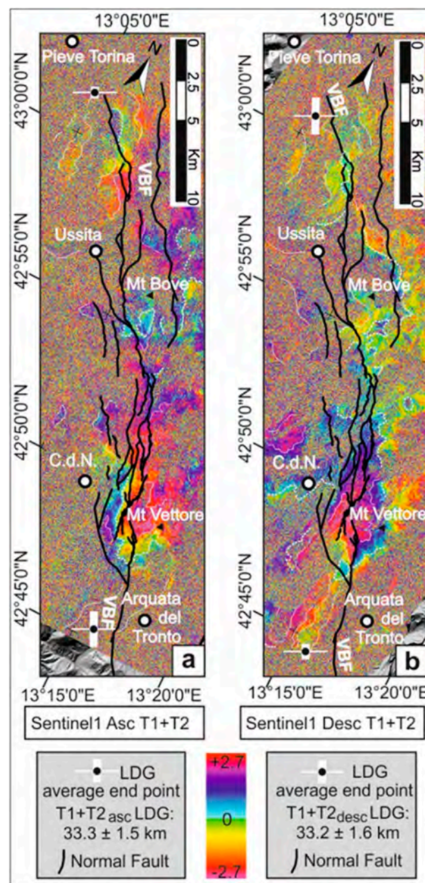
Figure 4. Same as Figure 3 but covering the entire period before the Mw 5.9 foreshock: T1+T2 period. (a) interferogram prepared from ascending orbit data between 27 August and 26 October, (b) interferogram prepared from descending orbit data between 2 September and 26 October.
