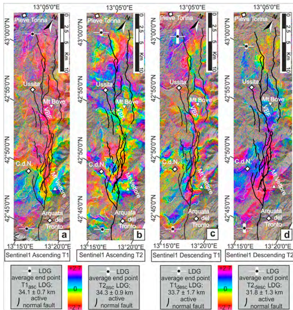
Figure 3. Phase changes detected before the occurrence of the Mw 5.9 foreshock during periods T1 (left) and T2 (right) as defined in text and Table 1. Interferograms were prepared using ESA Sentinel-1 images taken along relative ascending orbit 117 (a,b) and relative descending orbit 22 (c,d). We traced the interferometric fringes (white dotted lines) whose continuity is interrupted by low-coherence areas. The black dots mark endpoints of the segment delimiting the Length of Deforming Ground (LDG), and the corresponding white tapes show estimates of the endpoint location errors. One cycle of colors corresponds to one interferometric fringe (thicker white dotted lines) \sim 2.8 cm along the satellite Line of Sight (LoS). The thick black lines show the traces of the VBF. The colors show the patterns of phase changes around the VBF during the two intra-sequence periods, T1 and T2. C. d. N. = Castelluccio di Norcia.
