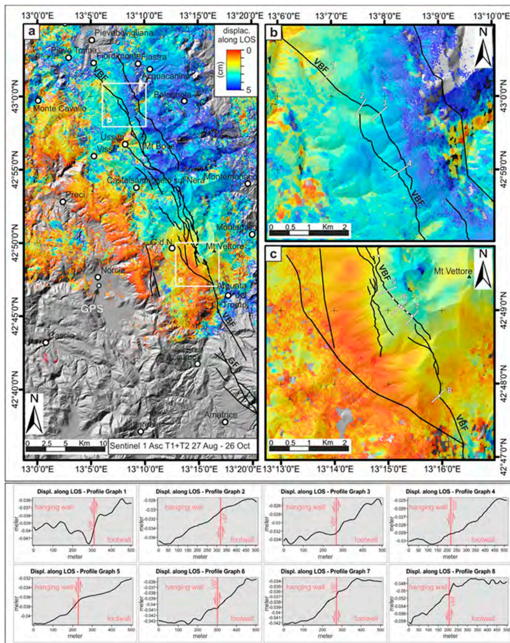
Figure 5. Displacement field obtained for the study area during the T1+T2 period along the ascending orbit. (a) Relative displacement field computed over high-coherence areas. The traces of the Vettore-Bove (VBF) and northern Gorzano (GF) fault are shown as black lines. (b,c) high-coherence sample areas selected to test the reliability of the observed displacement compared to the IGD detected in the interferograms of Figure 3 in the northern (b) and southern (c) sector of the VBF hanging wall and used to determine the Length of Deforming Ground (LDG). A coherence map of the area is provided in Figure S4a–c. The profiles (traces in b and c) show the displacements observed across the VBF whose intersection and sense of slip are indicated by the red vertical line.
