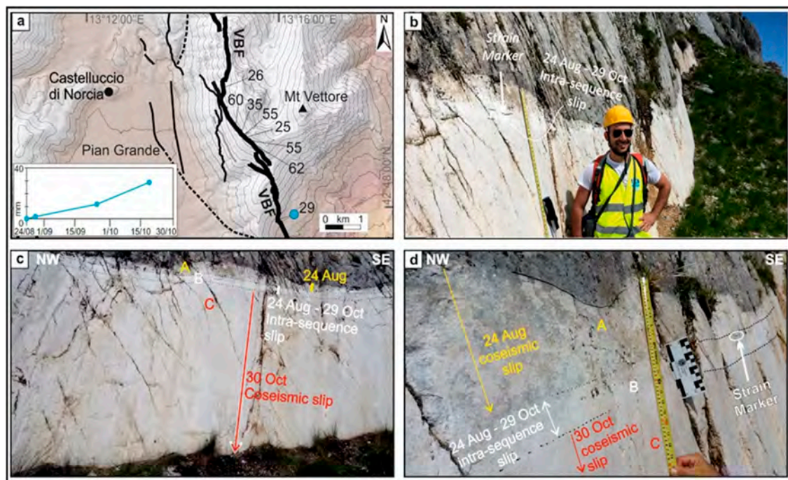
Figure 2. Field evidence of intra-sequence slip deformations along the Mt Vettore-Mt Vettoreto segment of the Mt Vettore-Mt Bove Fault (VBF), from 24 August to 29 October 2016. This fault segment was not reactivated during the Mw 5.9, 26 October event. (a) Location of survey sites where the total displacement due to Intra-sequence Ground Deformation (IGD, in mm) was measured on composite free faces. The inset shows the temporal trend of deformation where the VBF crosses Forca di Presta Provincial road SP34 (site #29). (b) Panoramic view of the free face exhumed along the VBF fault scarp (sites from #35 to #60). (c,d) Details of composite free faces documenting the 24 August-30 October slip-history along the VBF: (A) Upper band showing the coseismic slip caused by the 24 August Mw 6.0 foreshock; (B) Intermediate band showing the intra-sequence slip, between 24 August and 29 October 2016; (C) Lower (and thicker) band showing the coseismic deformation caused by the Mw 6.5 mainshock.
