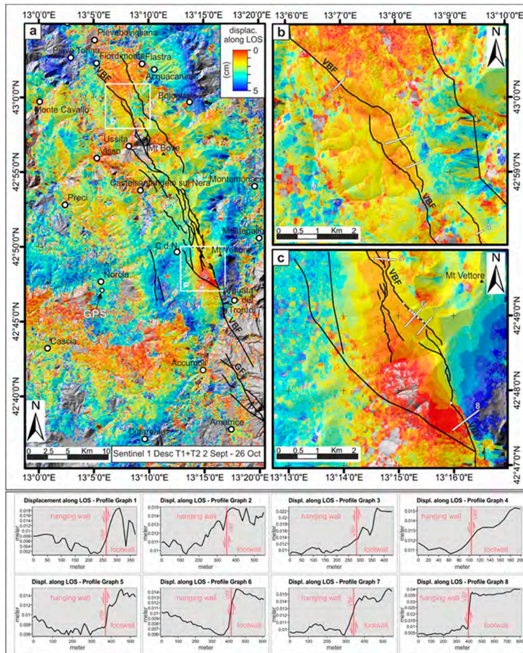
Figure 6. Same as Figure 5 but computed along the descending orbit. (a) Relative displacement field computed over high-coherence areas. The traces of the Vettore-Bove (VBF) and northern Gorziano (GF) fault are shown as black lines. (b,c) same high-coherence sample areas shown in Figure 5 showing results from the descending orbit. A coherence map of the area is provided in Figure S4d–f.
