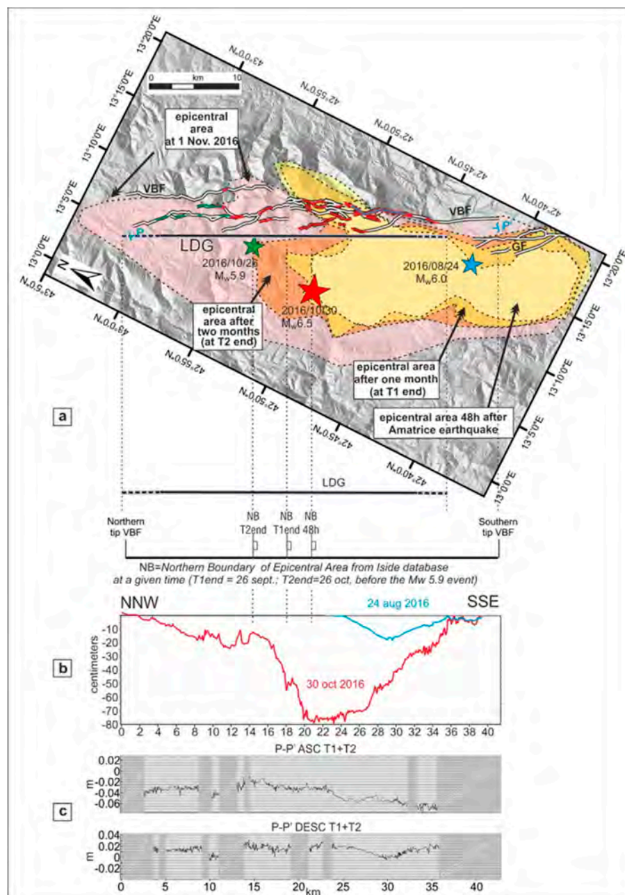
Figure 7. Coseismic and intra-sequence deformations compared to the spatial evolution of seismicity and major earthquake epicenters. (a) Map showing Length of Deforming Ground (LDG) (black-violet
